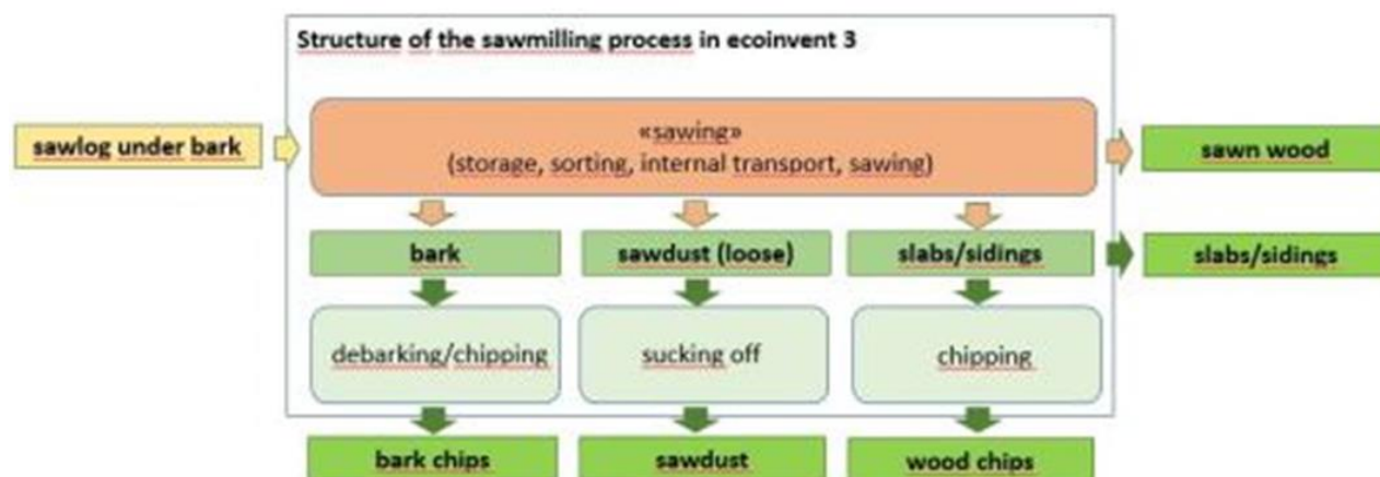
Figure 5. Structure of the sawmilling process in ecoinvent v3.2.
