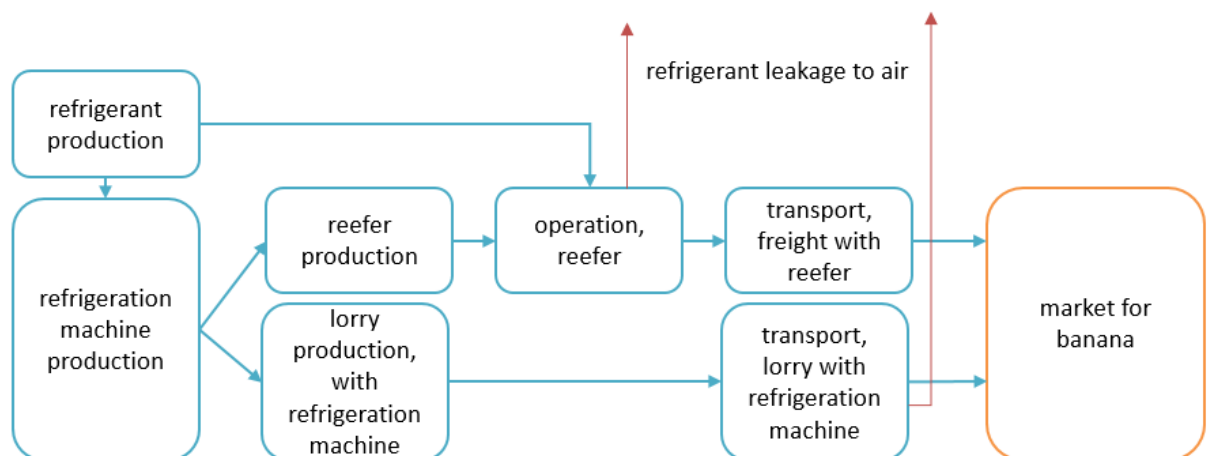
Figure 2. Scheme representing the relationship of the newly created datasets; transport of goods in need of atmosphere control
